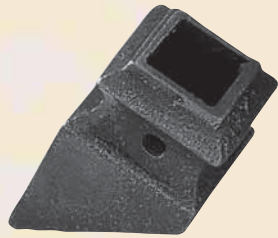
ART. PC60/1 MTL 1 3/16" x 1 31/32" SQ. MTL 9/16" HOLE FITS 1/2" BALUSTERS
