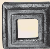
ART. PC60/8 MTL 2 23/64" SQ. MTL 1 1/4" HOLE FITS 1 3/16" NEWEL POSTS
